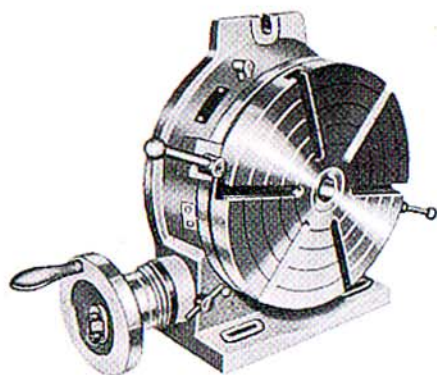
Horizontal Rotary Table (RT)
